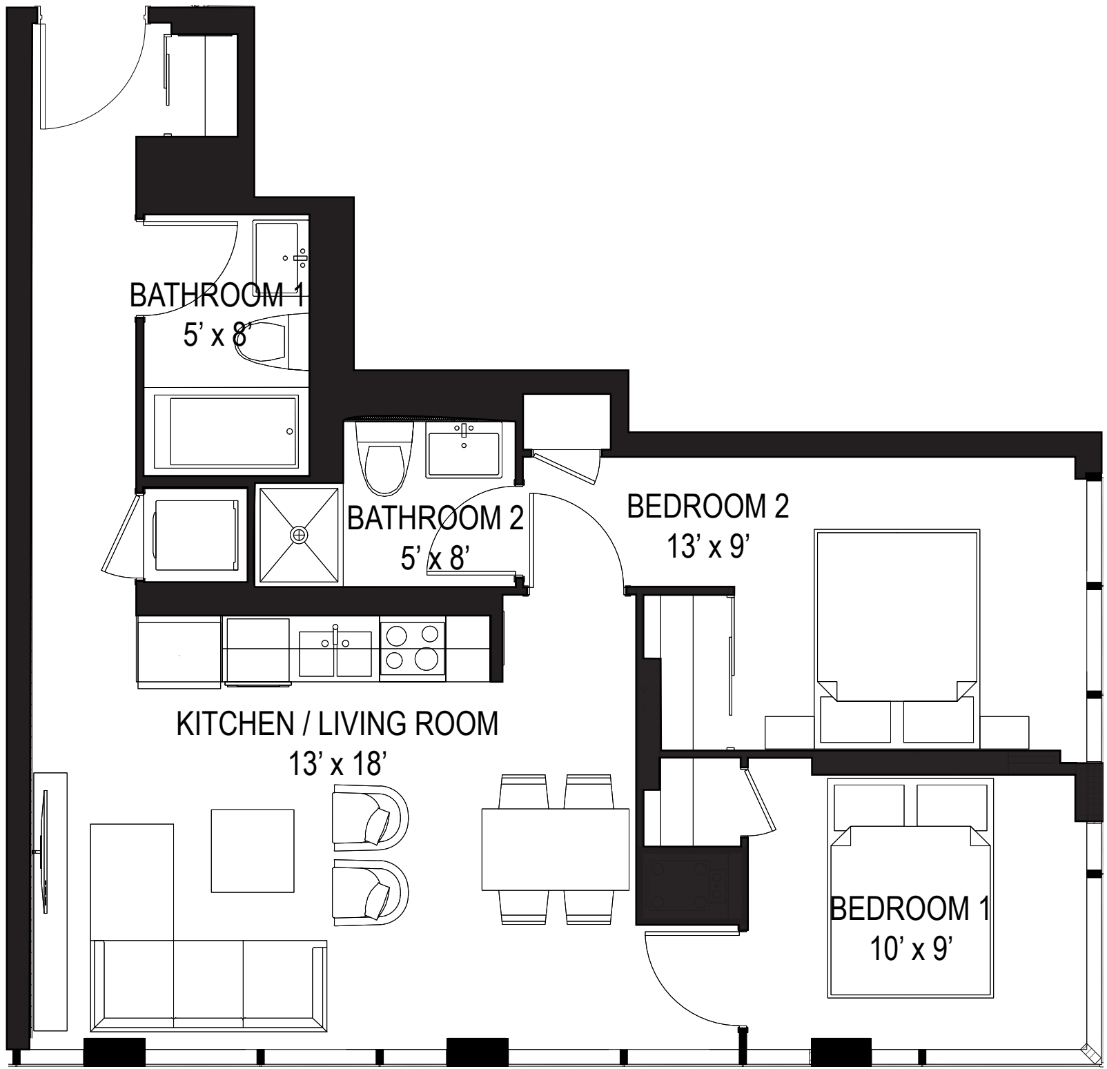
2-BEDROOM UNIT
